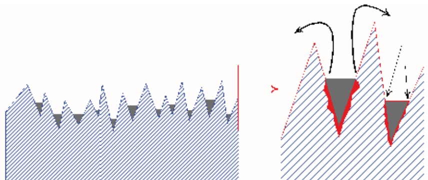
Fig. 9. Ground surface that has been significantly enlarged in the diagram. Dirt and other deposits ensure that chlorine ions, for example, are able to penetrate deeply underneath these depositions leading to local corrosion of the surface. Corrosion products such as rust will then appear.
